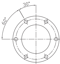
<6-HOLE FLANGE>
