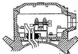
Terminal box for motor sizes 160 - 180
