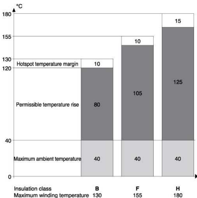
Safety margins per insulation class
