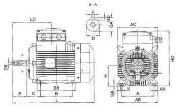
M2JA160-355
