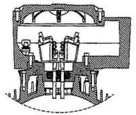
Terminal box for motor sizes 315 - 355
