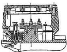
Terminal box for motor sizes 80 - 132
