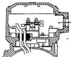
Terminal box for motor sizes 200 - 280
